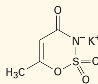
Acesulfame potassium
