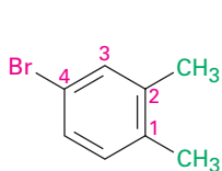
4-Bromo-1,2-dimethylbenzene
