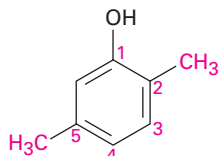
2,5-Dimethylphenol
