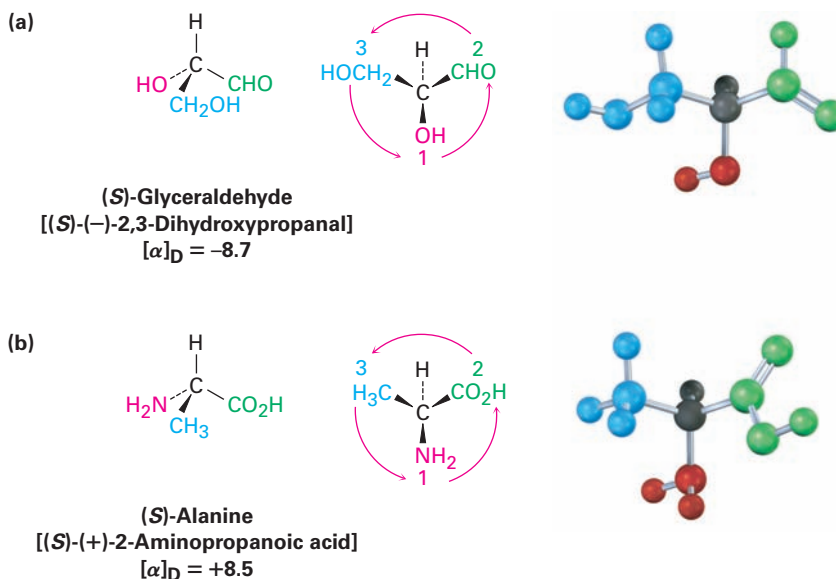
FIGURE 5-9 Assigning configuration to (a) (–)-glyceraldehyde. (b) (+)-alanine. Both happen to have the S configuration, although one is levorotatory and the other is dextrorotatory.
