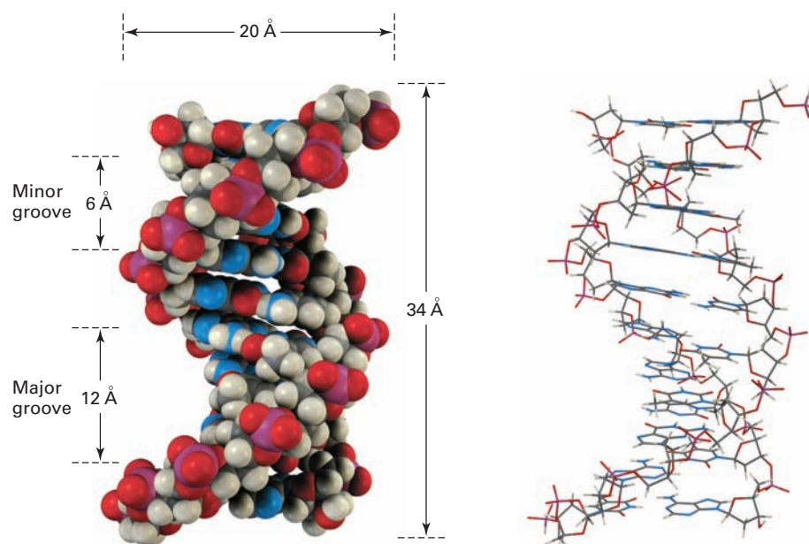
FIGURE 28-3 A turn of the DNA double helix in both space-filling and wire-frame formats. The sugar-phosphate backbone runs along the outside of the helix, and the amine bases hydrogen bond to one another on the inside. Both major and minor grooves are visible.
