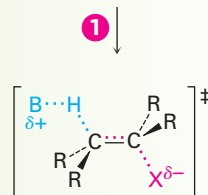
Transition state
