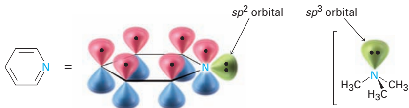
Pyridine
