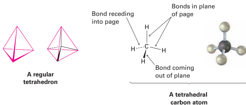
FIGURE 1-6 A representation of a tetrahedral carbon atom. The solid lines represent bonds in the plane of the page, the heavy wedged line represents a bond coming out of the plane of the page, and the dashed line represents a bond going back behind the plane of the page.
