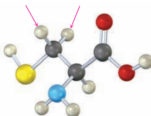
Cysteine
