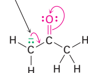
Acetone anion (two resonance forms)
