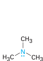
Trimethylamine
