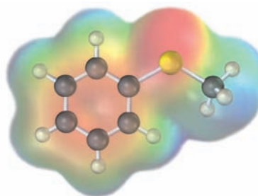
Thioanisole ( \text{C}_6\text{H}_5\text{SCH}_3 )
