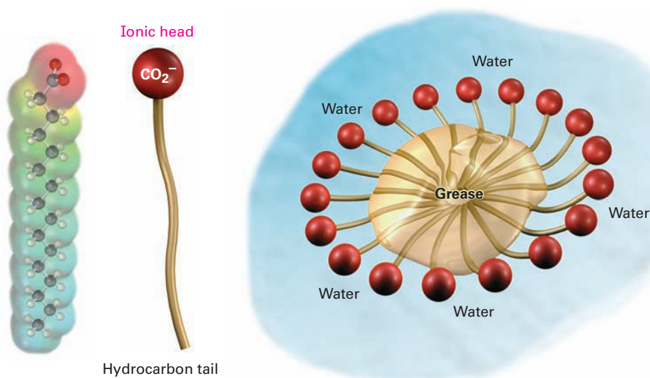
FIGURE 27-1 A soap micelle solubilizing a grease particle in water. An electrostatic potential map of a fatty acid carboxylate shows how the negative charge is located in the head group.
