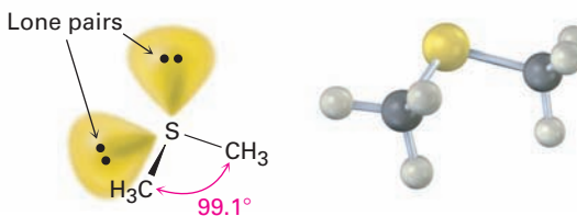
Dimethyl sulfide
