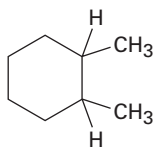
1,2-Dimethylcyclohexane
