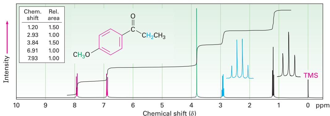
FIGURE 13-10 The ^1\text{H} NMR spectrum of para -methoxypropiphenone.
