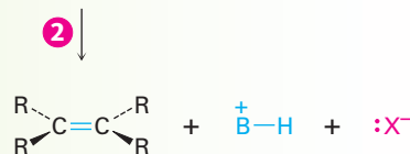
Transition state
