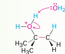
Protonated alcohol
