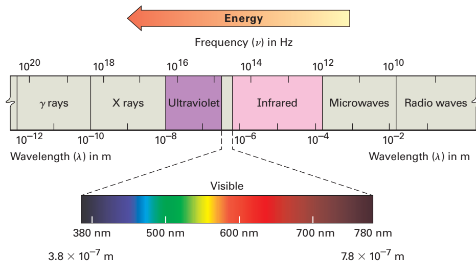
FIGURE 12-16 The electromagnetic spectrum covers a continuous range of wavelengths and frequencies, from radio waves at the low-frequency end to gamma ( \gamma ) rays at the high-frequency end. The familiar visible region accounts for only a small portion near the middle of the spectrum.
