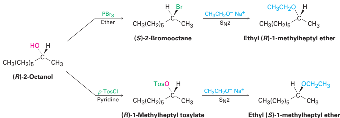
FIGURE 17-5 Stereochemical consequences of \text{S}_{\text{N}}2 reactions on derivatives of ( R )-2-octanol. Substitution through the halide gives a product with the same stereochemistry as the starting alcohol; substitution through the tosylate gives a product with opposite stereochemistry to the starting alcohol.
