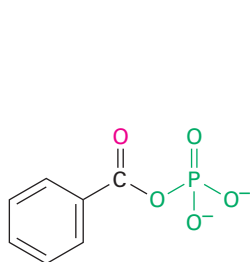
Benzoyl phosphate
