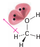
Methanol ( \mu = 1.70 D)
