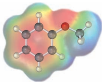
Anisole ( \text{C}_6\text{H}_5\text{OCH}_3 )
