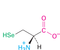
Selenocysteine
