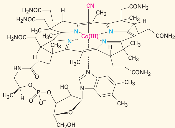
Vitamin B 12
