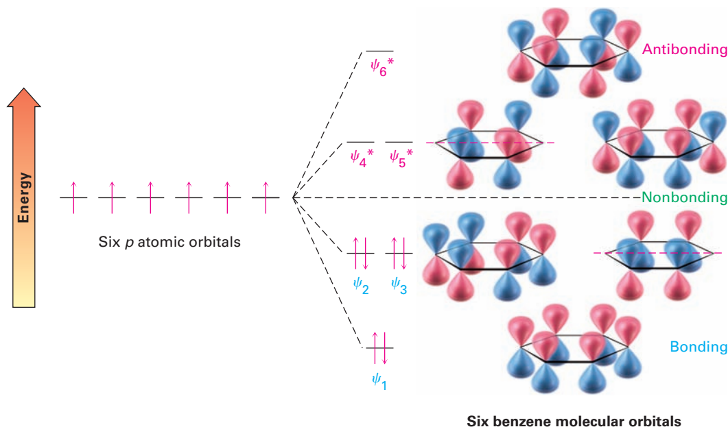
FIGURE 15-4 The six benzene \pi molecular orbitals. The bonding orbitals \psi_2 and \psi_3 have the same energy and are said to be degenerate , as are the antibonding orbitals \psi_4^* and \psi_5^* . The orbitals \psi_3 and \psi_4^* have no \pi electron density on two carbons because of a node passing through these atoms.
