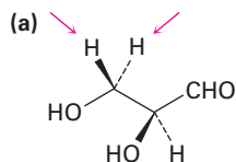
(S)-Glyceraldehyde
