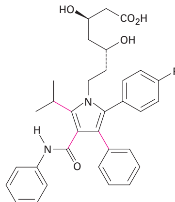
Atorvastatin (Lipitor)
