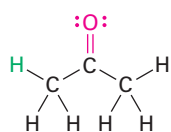
Acetone
