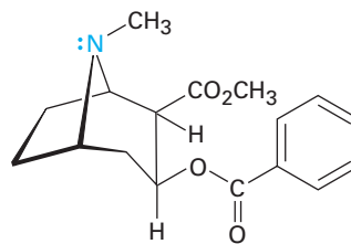
Cocaine
