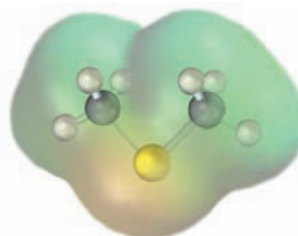
Ether
