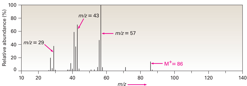
FIGURE 12-5 Mass spectrum of hexane ( \text{C}_6\text{H}_{14} ; MW = 86). The base peak is at m/z = 57 , and numerous other ions are present.
