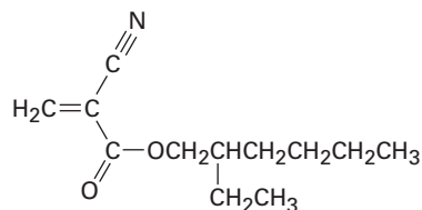
Methyl \alpha -cyanoacrylate
