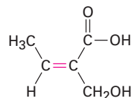
( Z )-2-Hydroxymethyl-2-butenoic acid
