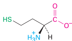
Homocysteine
