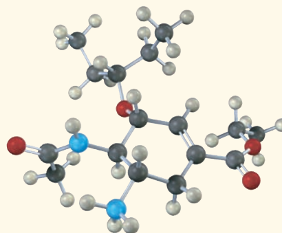
FIGURE 4-18 The structure of Tamiflu (oseltamivir), an antiviral agent active against type A influenza, and a molecular model of its minimum-energy conformation as calculated by molecular mechanics.
