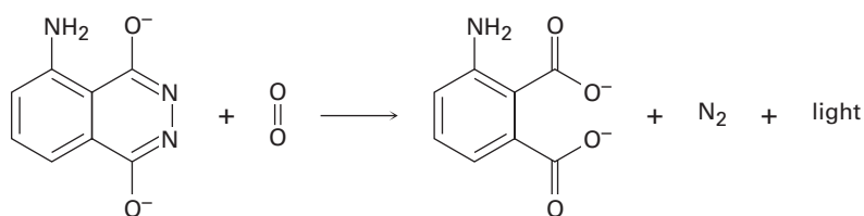
Luminol dianion
