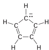
Cyclopentadienyl anion
