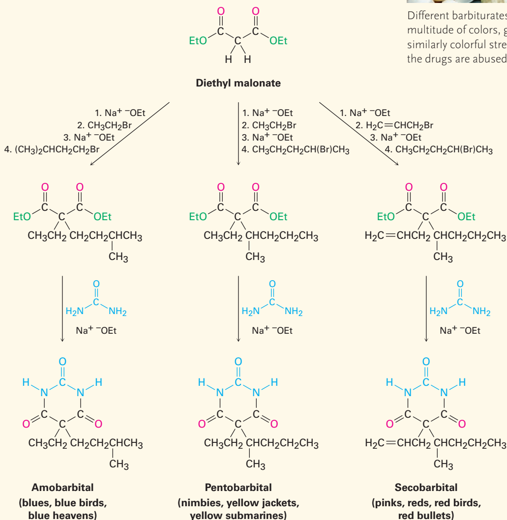
FIGURE 22-7 The synthesis of barbiturates relies on malonic ester alkylations and nucleophilic acyl substitution reactions. More than 2500 different barbiturates have been synthesized over the past 100 years. In addition to their legal medical uses, some barbiturates are also used illegally as street drugs under many colorful names.
