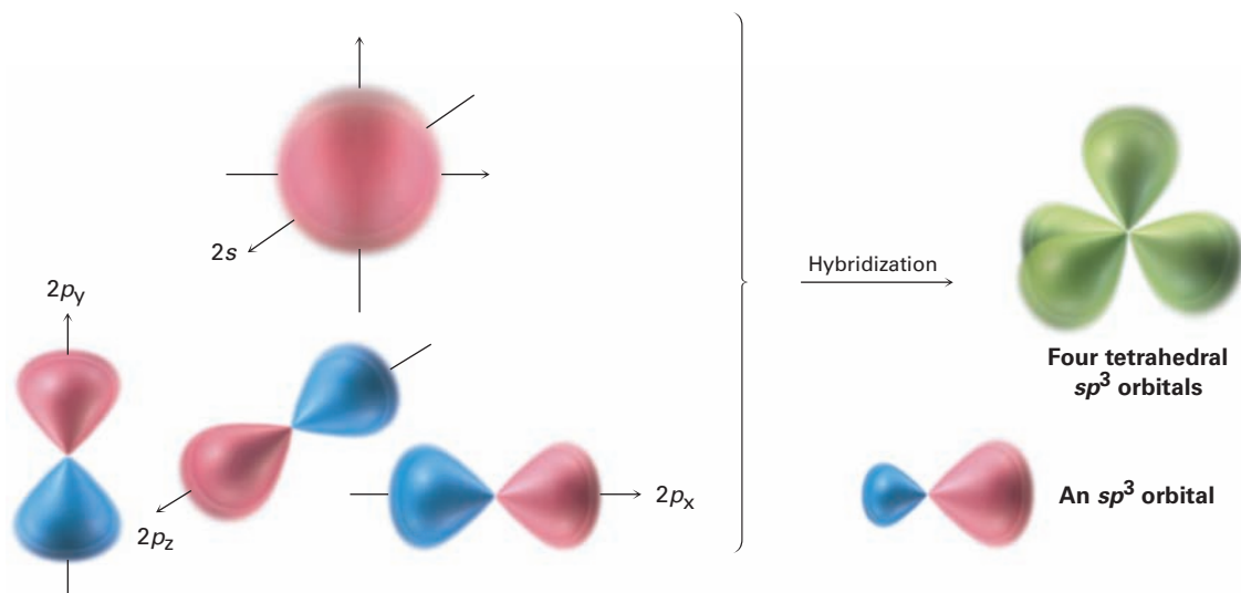
FIGURE 1-10 Four sp^3 hybrid orbitals, oriented to the corners of a regular tetrahedron, are formed by the combination of an s orbital and three p orbitals. The sp^3 hybrids have two lobes and are unsymmetrical about the nucleus, giving them a directionality and allowing them to form strong bonds when they overlap an orbital from another atom.
