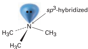
Trimethylamine
