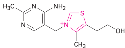
Thiazolium ring
