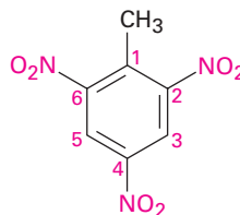
2,4,6-Trinitrotoluene (TNT)
