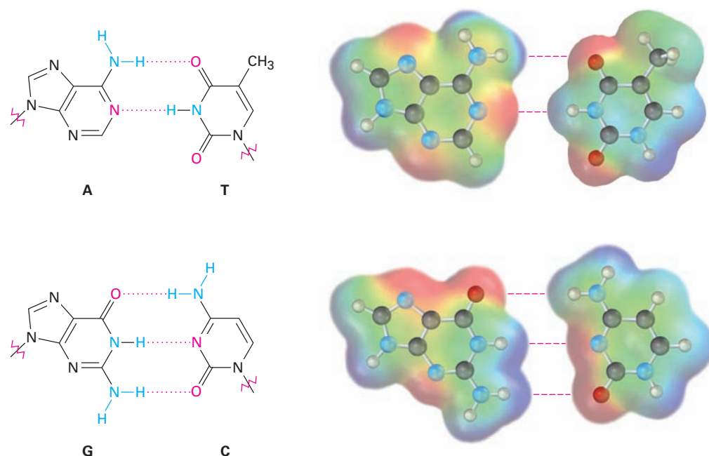
FIGURE 28-2 Hydrogen-bonding between base pairs in the DNA double helix. Electrostatic potential maps show that the faces of the bases are relatively neutral ( green ), while the edges have positive and negative regions. Pairing G with C and A with T brings together oppositely charged regions.
