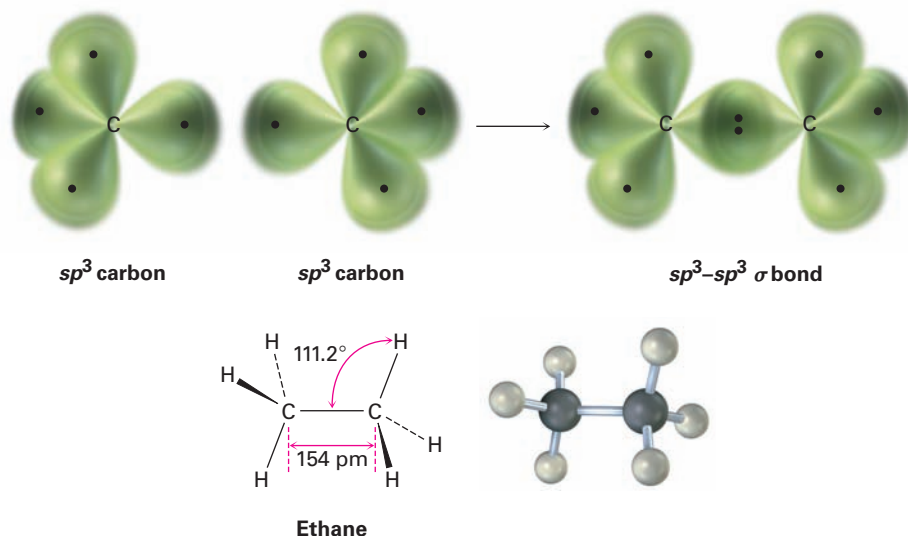
FIGURE 1-12 The structure of ethane. The carbon–carbon bond is formed by \sigma overlap of sp^3 hybrid orbitals. For clarity, the smaller lobes of the sp^3 hybrid orbitals are not shown.
