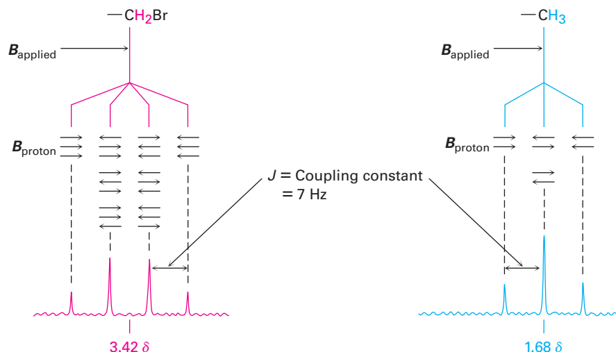
FIGURE 13-8 The origin of spin-spin splitting in bromoethane. The nuclear spins of neighboring protons, indicated by horizontal arrows, align either with or against the applied field, causing the splitting of absorptions into multiplets.
