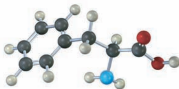
Phenylalanine
