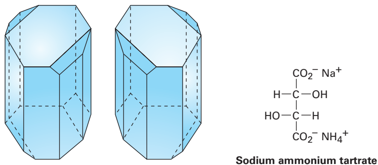
FIGURE 5-6 Drawings of sodium ammonium tartrate crystals taken from Pasteur's original sketches. One of the crystals is dextrorotatory in solution, and the other is levorotatory.
