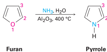
Furan
