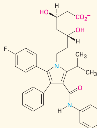
Atorvastatin (Lipitor)
