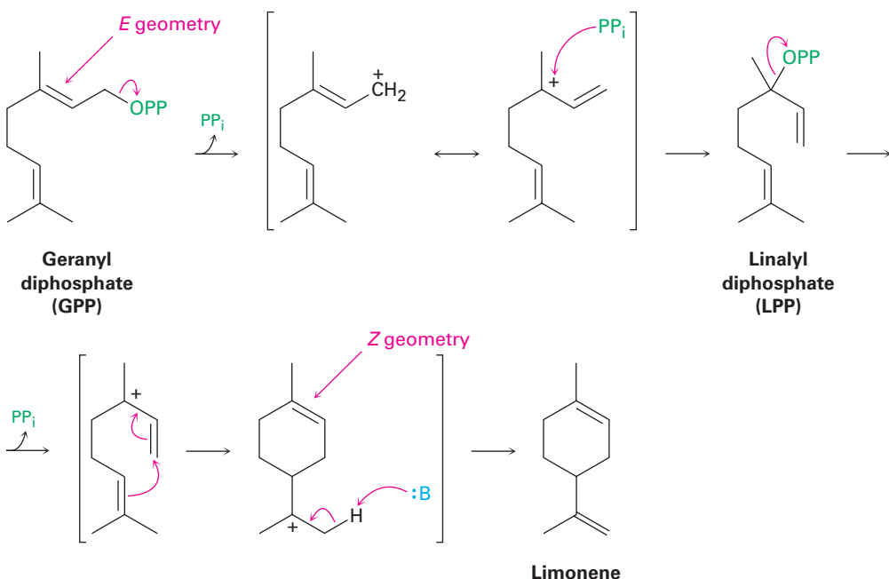
FIGURE 27-10 Mechanism for the formation of the monoterpene limonene from geranyl diphosphate.
