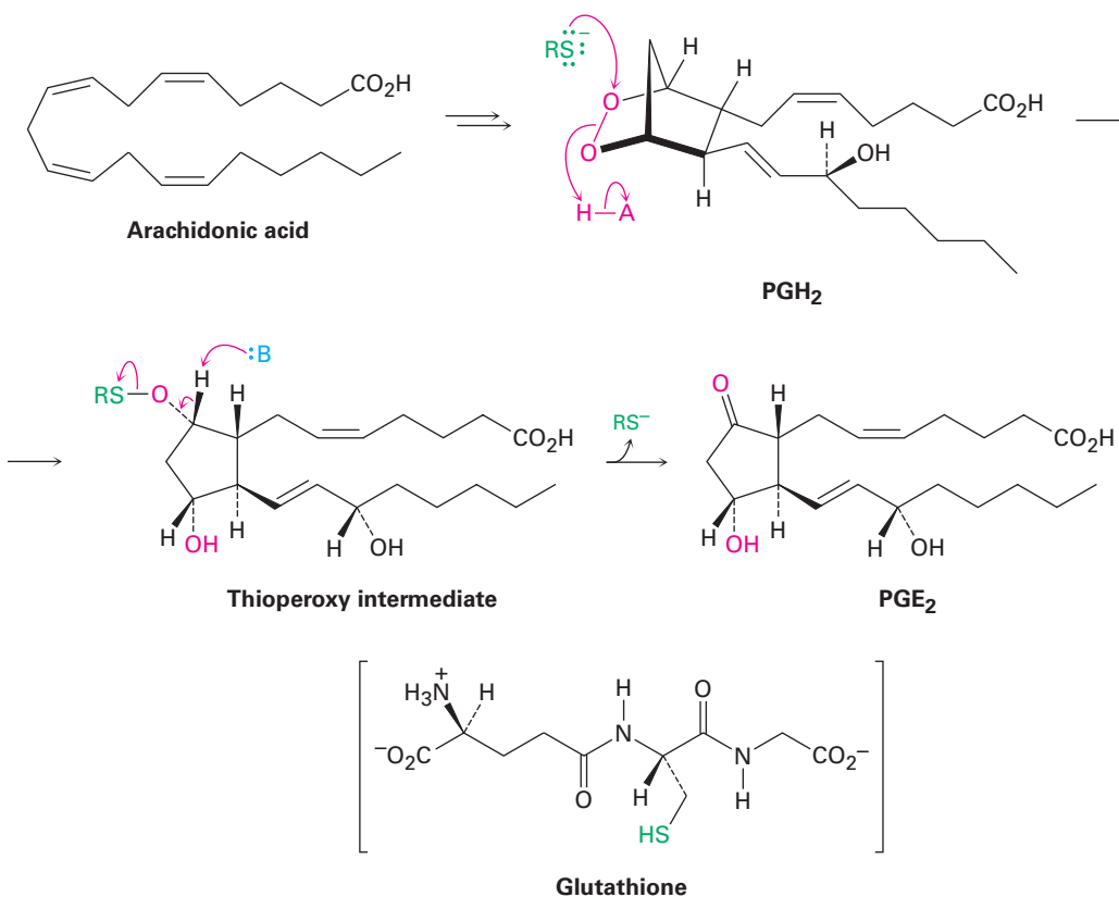
FIGURE 27-5 Mechanism of the conversion of PGH 2 into PGE 2 .
